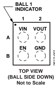
Figure 2. Pin Configuration
